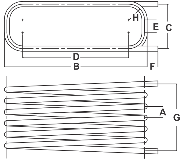
RECTANGULAR BOX COIL
